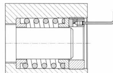
Pre-loading or relief setting of a spring mounted device inside a housing.
