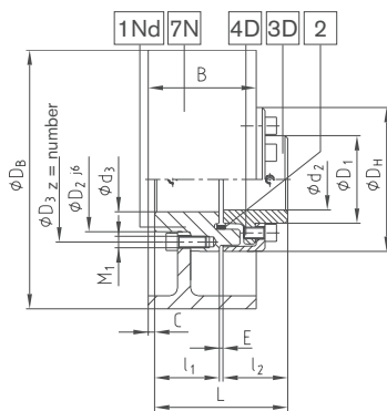
Brake drum type ADR-BTA
