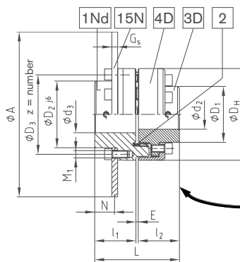
Brake disk type ADR-SBA
